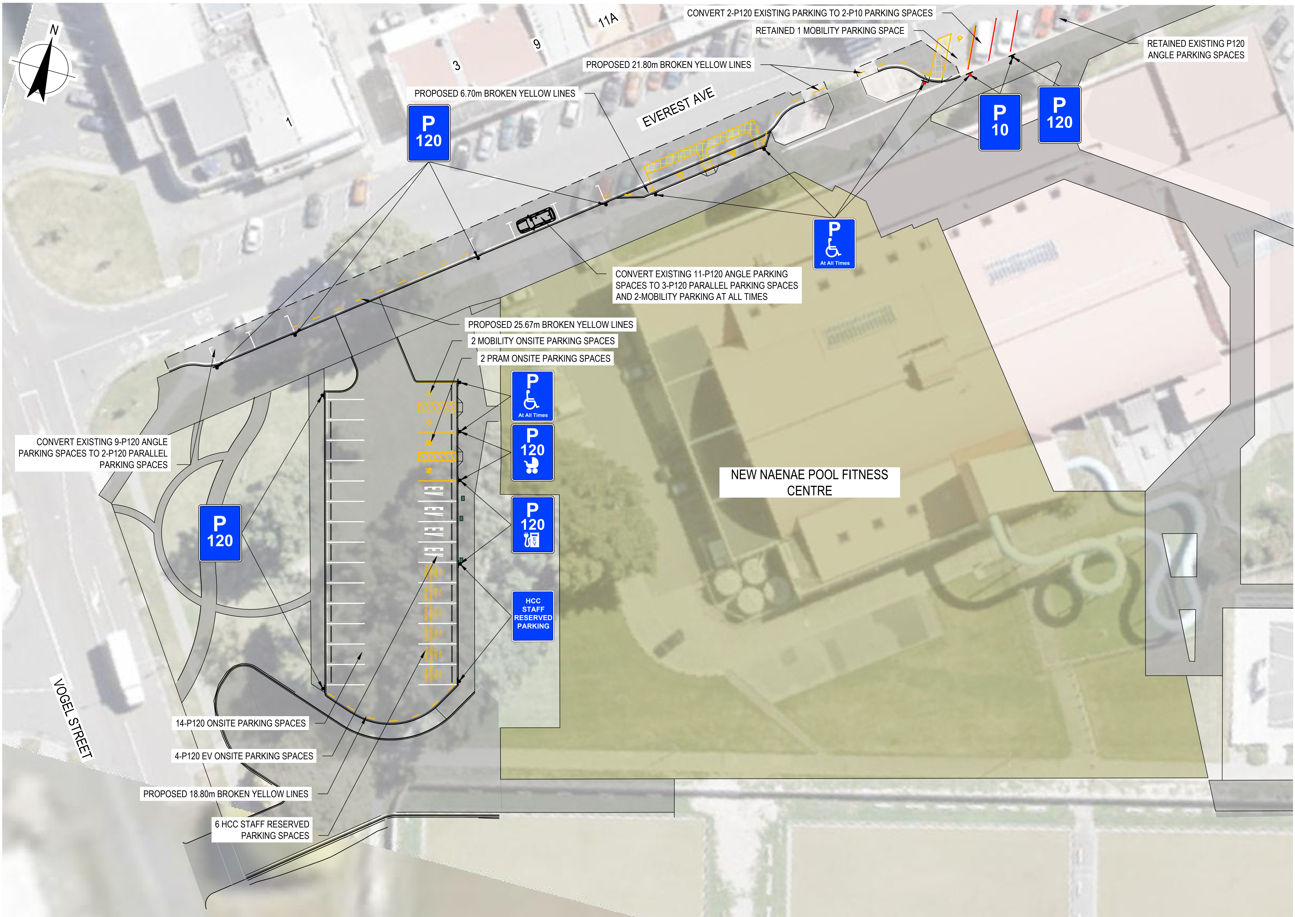
PLAN SCALE 1:250
