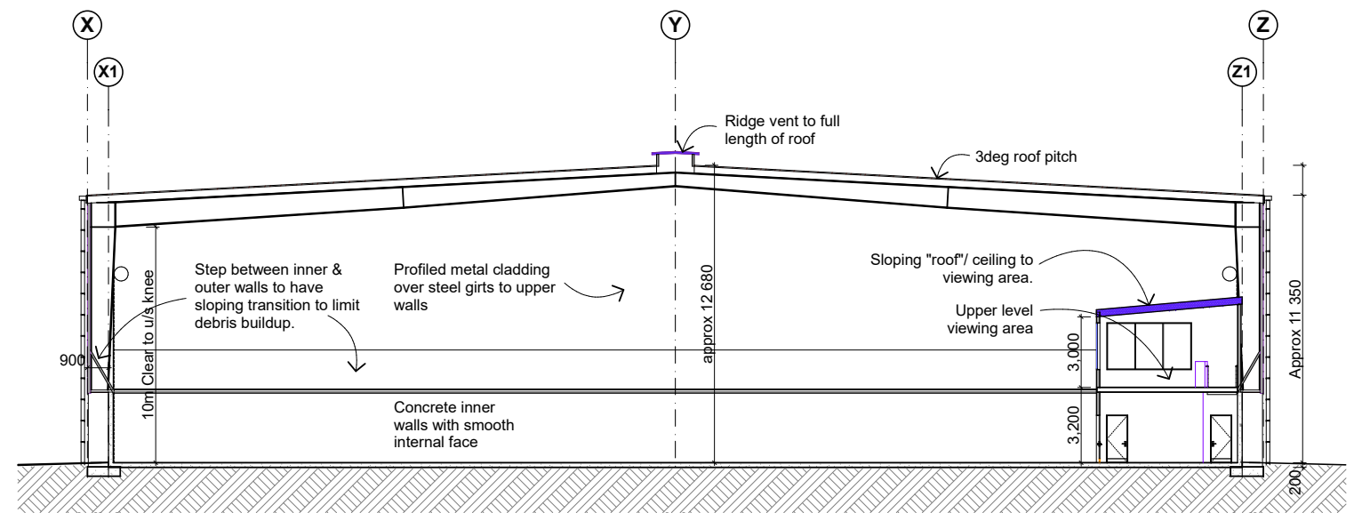
Cross Section
