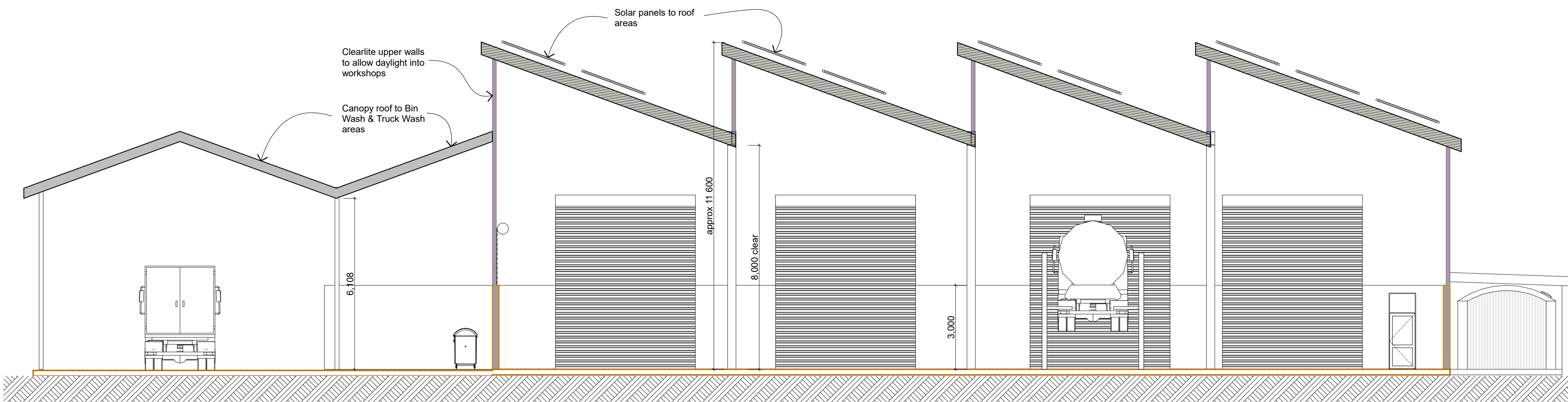
Long Section
