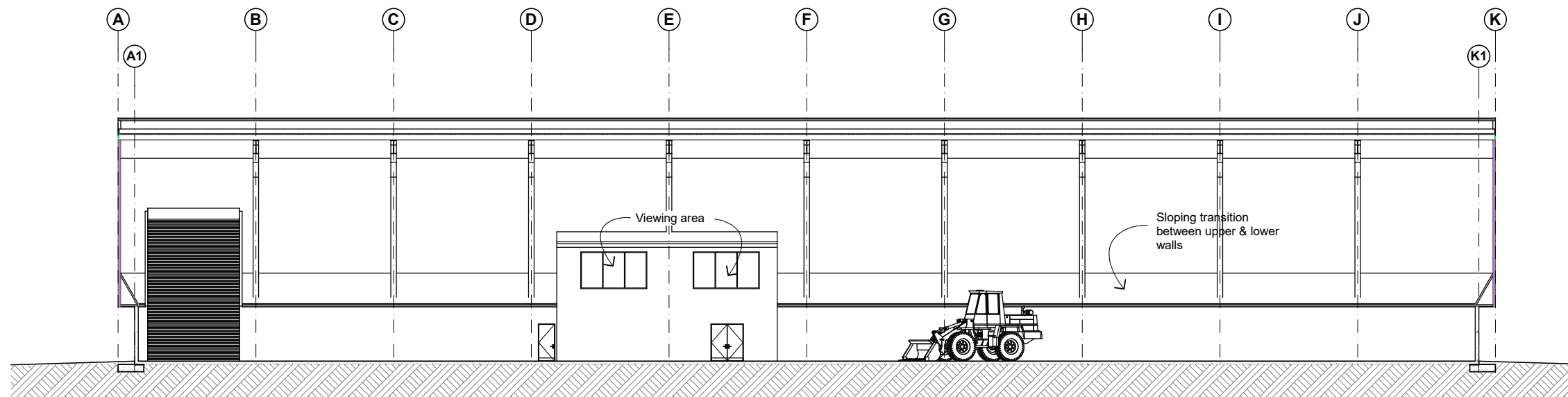
Long Section
