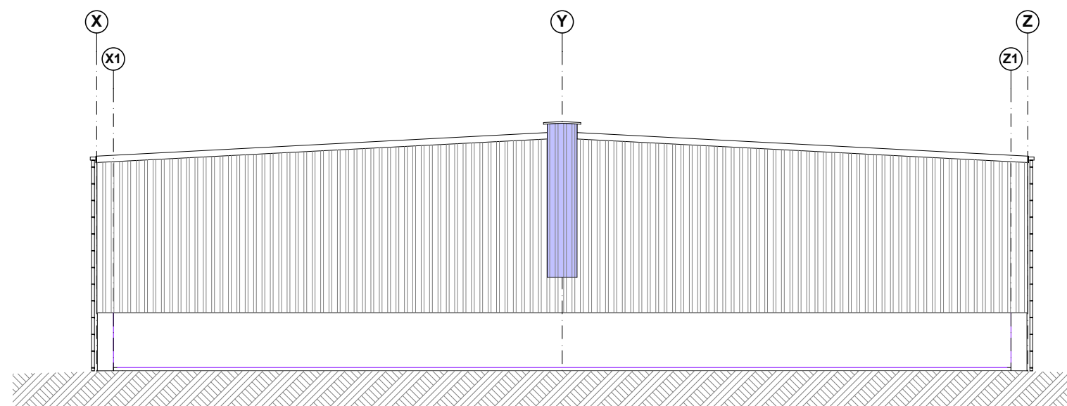
East Elevation
